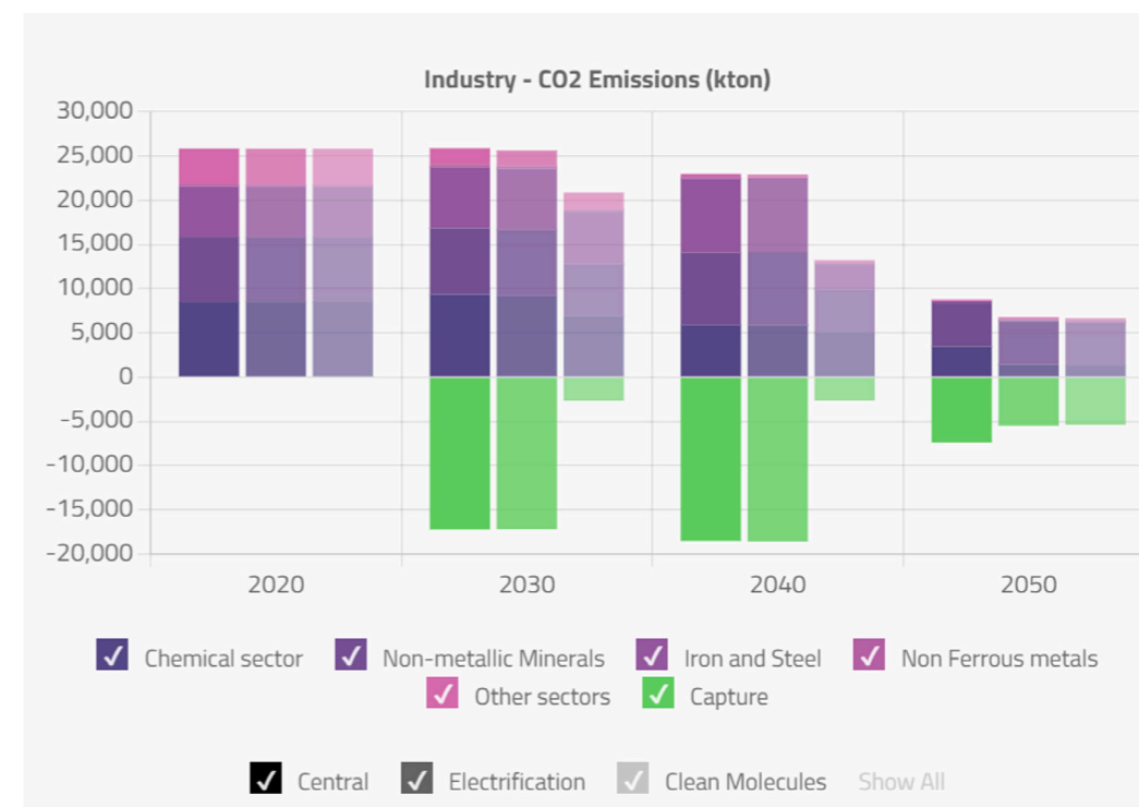
Figure 28. Total industry CO 2 emissions by scenario from 2020 to 2050.
