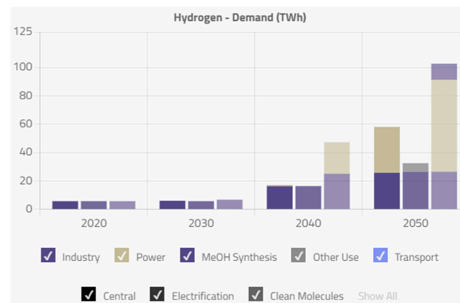
Figure 37. Hydrogen demand by final use.
