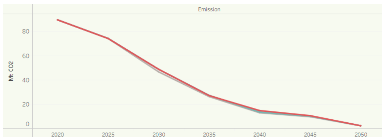
Figure 5: Emission savings of the defined scenarios, total emission of the system, not only electricity production. Emissions of the scenario with both D4/T3 extended as D3/T2 restarted (brown line) has slightly lower emissions than the lifetime extension of D4/T3 for 20 years (blue line) and for 10 years (red line). The maximum difference is 2.1 Mt in 2030, (only the effect of restarting D3/T2). In 2040, extending D4/T3 and D3/T2 for 20 years has 1.8Mt less emissions than the base scenario where only D4/T3 is extended for 10 years.
